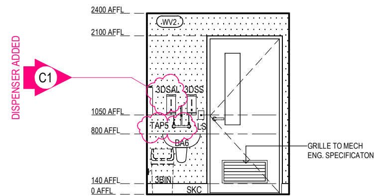
RACF BOH - CLEANER - TYPE 1 ELEVATION 1 Scale 1 : 50
