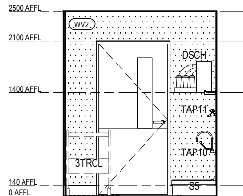
RACF BOH - CLEANER - TYPE 2 ELEVATION 4 Scale 1 : 50
