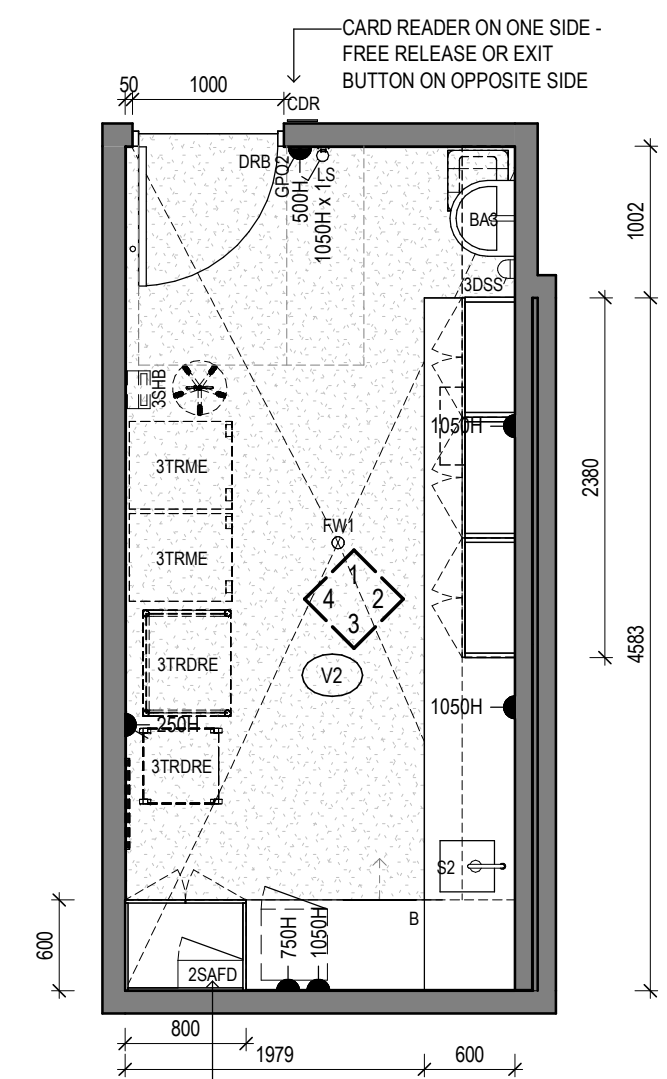
5 RACF-TREATMENT Scale 1 : 50
