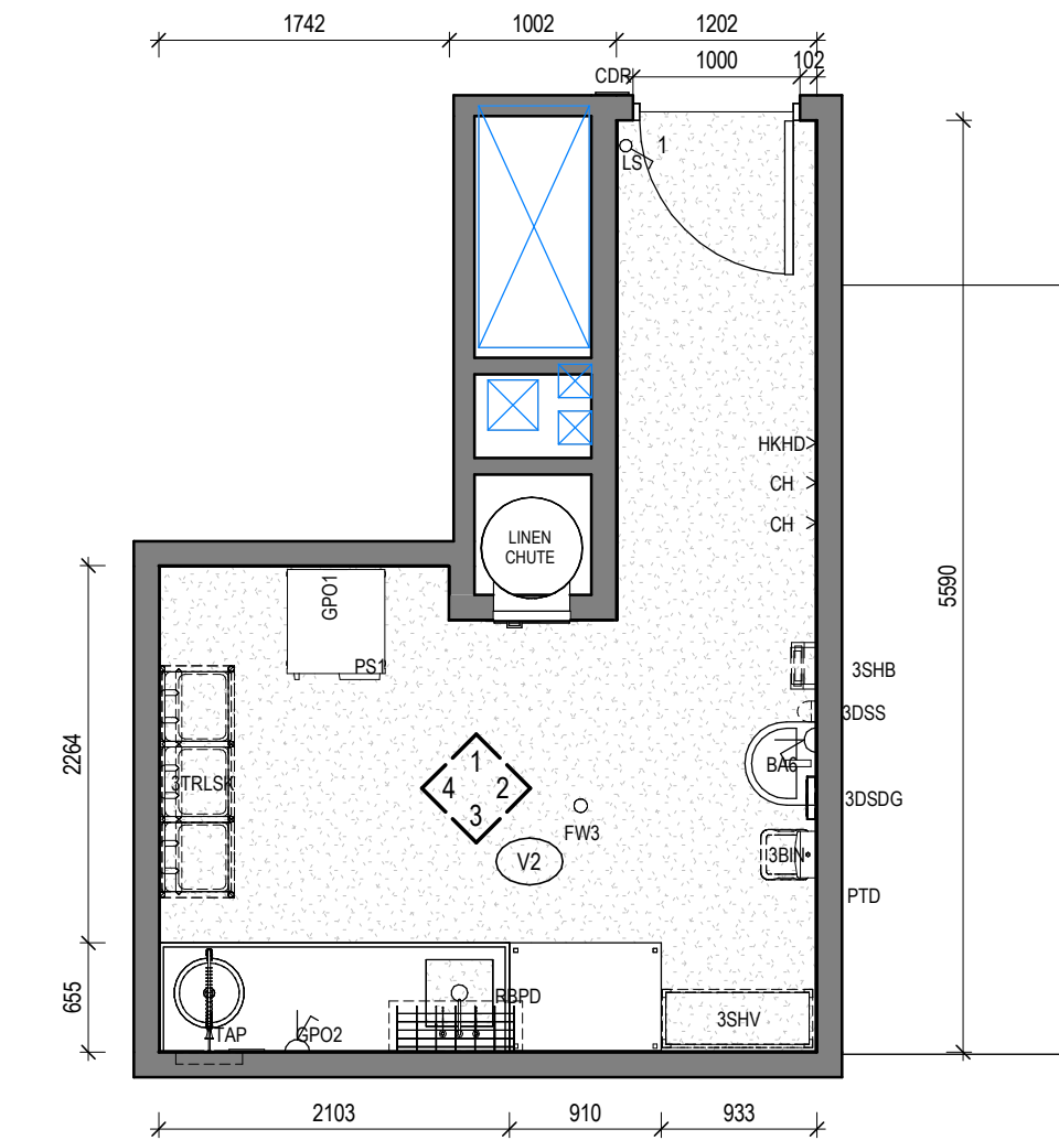
7 RACF-SLUICE Scale 1 : 50
