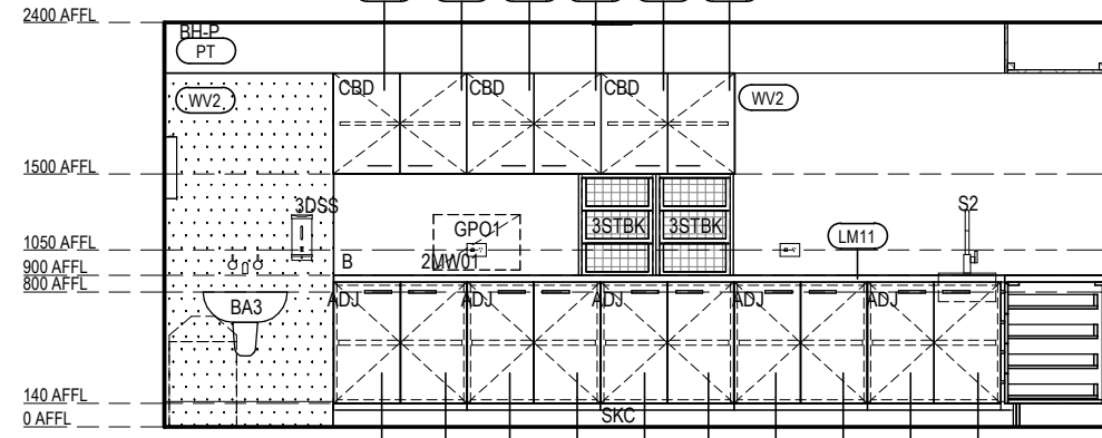
RACF BOH - TREATMENT ELEVATION 2 Scale 1 : 50
