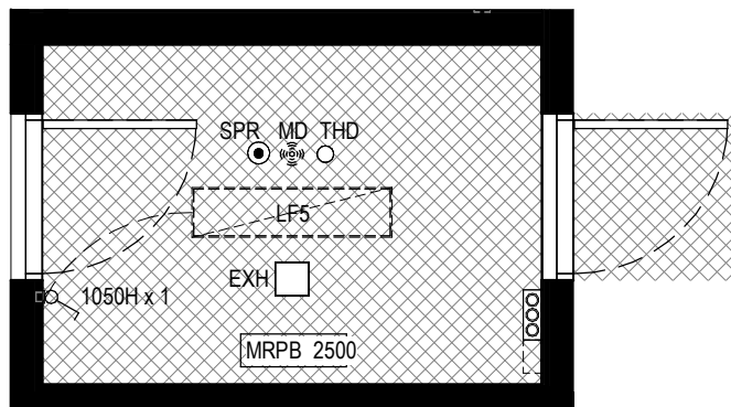
4 RCP-CLEANER - TYPE 2 Scale 1 : 50
