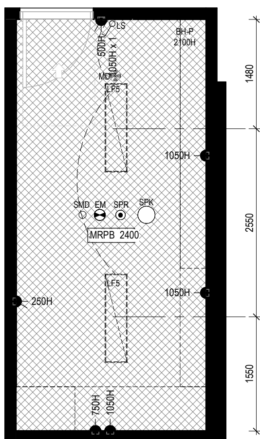
6 RCP-TREATMENT Scale 1 : 50
