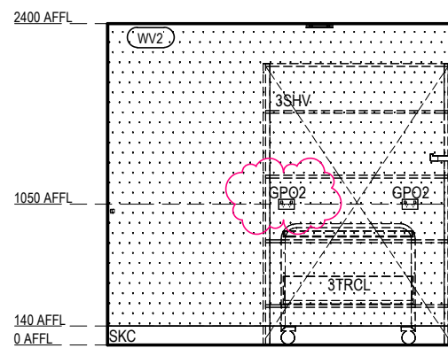
RACF BOH - CLEANER - TYPE 1 ELEVATION 2 Scale 1 : 50
